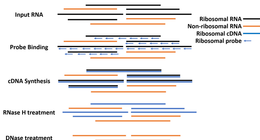
Fig. 1. Workflow for reverse-transcriptase mediated ribosomal depletion from total RNA. To perform ribosomal RNA (rRNA) depletion, total RNA is first extracted, DNase treated and subsequently purified with RNAClean XP Beads (Agencourt). DNA-free RNA is then bound to oligonucleotide probes designed to bind to rRNA from mosquito species in Aedes , Culex and Anopheles genera that are in the reverse complement orientation to both the long and short ribosomal subunit and 12S and 16S mitochondrial rRNA. The RNA with bound oligos is then subjected to reverse transcription using Avian Myeloblastosis Virus (AMV) Reverse Transcriptase (NEB). RNA that is reverse transcribed to cDNA is then digested using RNase H, which selectively destroys RNA in an RNA:DNA hybrid. Remaining DNA is then digested using DNase I (NEB), leaving mostly non-ribosomal RNA which is then used for library preparation.
