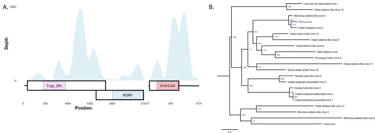
Fig. 10. Description of a novel Luteo-Sobemo like virus from Aedes aegypti mosquitoes. A- Cartoon depicting the predicted bipartite genomic structure of RENV. Large boxes represent ORFs, small boxes represent areas of protein homology to Trypsin-like serine protease (cd00190), viral RNA-dependent RNA polymerase (cd1699), and capsid protein (cd00205). B- Phylogenetic placement of RENV. Phylogeny was created using a 289 amino acid portion of the RDRP. Trees are midpoint rooted. Bootstrap proportions are shown for each node. Phylogenetic trees were viewed in FigTree.
