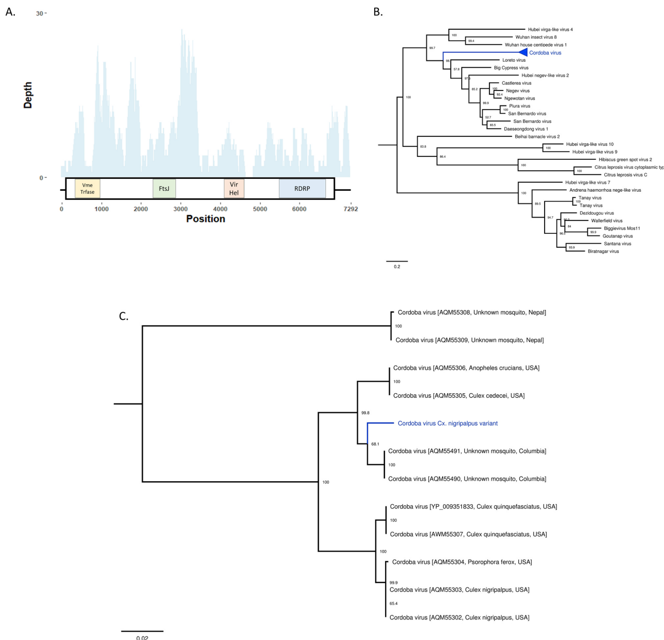
Fig. 8. Description of a novel variant of the negevirus Cordoba virus from Culex nigripalpus A- Virus cartoon depicting the genomic structure and depth of coverage Cordoba virus Cx. nigripalpus variant. The large boxes represent predicted ORFs and the small boxes represent areas of protein homology to viral methyltransferase (pfam01660), FtsJ-like methyltransferase (pfam01728), viral RNA helicase (pfam01443), and viral RNA-dependent RNA polymerases (cd1699). B. Phylogenetic placement of multiple strains of Cordoba virus highlighted in blue. Phylogenies were created using 1234 A.A. residues across the complete ORF. Tree is midpoint rooted. Phylogenetic trees were generated in FigTree. C. Expansion of phylogenetic tree containing the sequenced strains of Cordoba virus. The strain sequenced in this study is highlighted in blue. Bootstrap proportions are shown for each node. Phylogenetic trees were viewed in FigTree.
