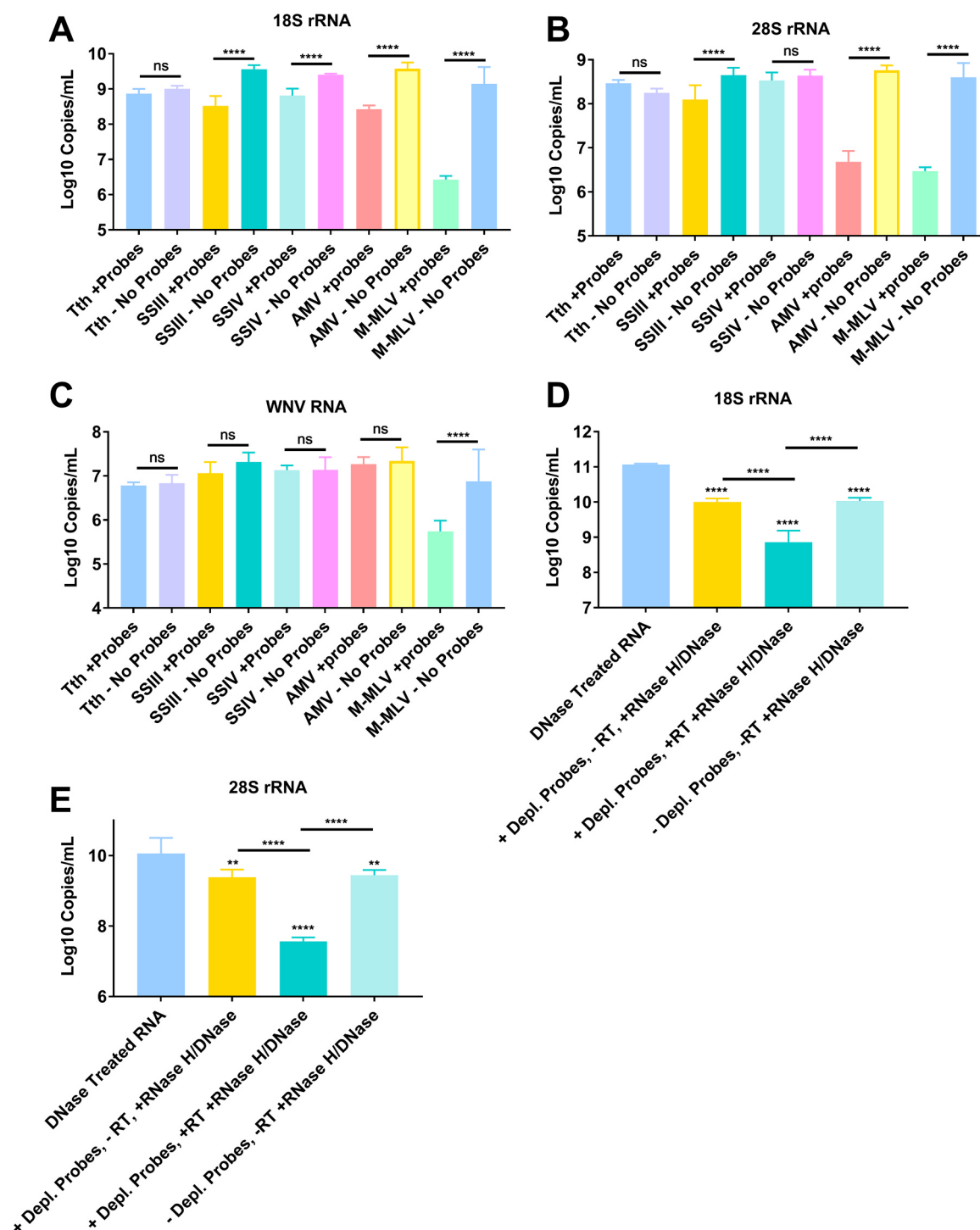
Fig. 2. Reverse Transcriptase mediated ribosomal RNA (rRNA) depletion is most effective with AMV RT and requires all steps to be effective. Nucleic acids were eluted from FTA cards with midgut contents of An. gambiae that had been exposed to a bloodmeal containing West Nile virus (WNV) placed on them. RNA and DNA was then extracted to obtain total nucleic acid. The nucleic acid was then treated with DNase I and then purified to obtain total RNA. This RNA was then subjected to cDNA synthesis with a panel of reverse transcriptases ( n = 3 for each treatment) in the presence (+ probes) or absence (- probes) of DNA probes specific to rRNA. The RTs tested were Tth DNA polymerase, Superscript III (SSIII), Superscript IV (SSIV), AMV and MMLV. All the samples were then treated with RNase H and then DNase I to remove the RNA present in an RNA:DNA hybrid and cDNA, respectively. The samples were then purified and subjected to qRT-PCR with primer probe combinations specific for 18S rRNA (A), 28S rRNA (B) or WNV (C). Further tests were performed exclusively with AMV RT. Panels D and E show the results of qRT-PCR for samples that underwent the process of depletion but omitting some step or reagent. 18S (D) and 28S (E) rRNA was quantified in the input RNA, RNA with no RT added, RNA with no depletion probes added and RNA treated with RT with depletion probes. All statistical tests were performed by One-Way ANOVA with Tukey test for multiple comparisons. ****Indicates p -value < 0.0001 . All stars without an accompanying bar are statistical comparisons between the DNase Treated RNA and the other group. The other comparisons with a bar are statistical comparisons between the two groups that are below the corresponding bar.
