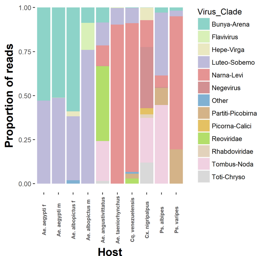
Fig. 7. Viral sequences belonging to diverse clades of RNA viruses identified in field-collected mosquitoes following rRNA depletion. Individual reads from each mosquito species sequenced were mapped back to all virus contigs identified in this study. Virus clade is inferred by amino acid similarity to other closely related sequences. The total number of reads aligning to each virus clade was graphed as a proportion of the total number of viral reads produced from each mosquito species.
